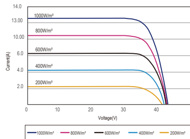
I-V Curves(550W)
